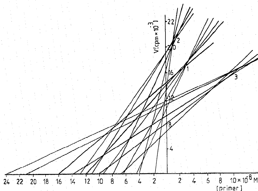
Fig. 2. Initial rate of polymerization catalyzed by AMV-RT versus concentrations of d(pT)_8 (1), Chs- d(pT)_8 (2) and Phn- d(pT)_8 (3) in the Cornish-Bowden and Eisenthal coordinates.
